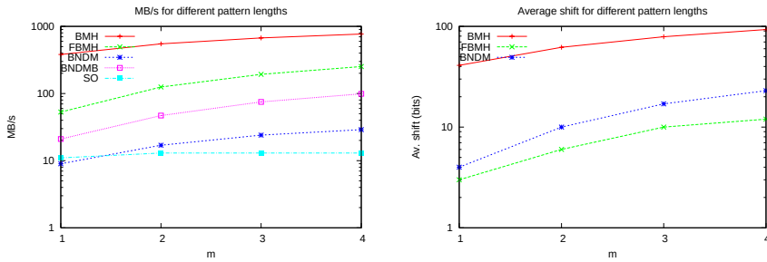
Fig. 1. Search performance. Left: MB/second processed by different algorithm. Right: the average shift in bits. The x -axis ( m ) is the pattern length in words.
