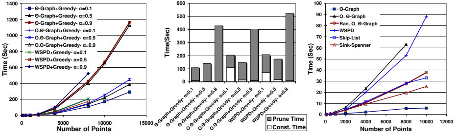
Fig. 2. (a) The performance of the hybrid algorithms for different values of \alpha (Uniform distr. and t = 2 ). (b) Comparing the construction time of the initial graph with the pruning time (Uniform distr., t = 2 and n = 8000 ). (c) The running time for the \mathcal{O}(n \log n) -time algorithms in the experiments for Uniform distr. with t = 1.1 .
