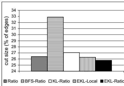
(a) Average percentage of edges in cuts found by each heuristic.
