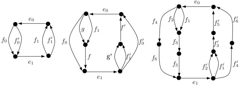
Fig. 1. Network Constructions \mathcal{G}_1 , \mathcal{G}_2 , and \mathcal{G}_3
