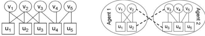
(a) Graph G constructed from the (b) Optimal partitioning of G for cooperative system of equations (3). 2-agent problem solving.
