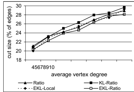
(b) Average percentage of edges in cuts found by each heuristic versus average vertex degree.
